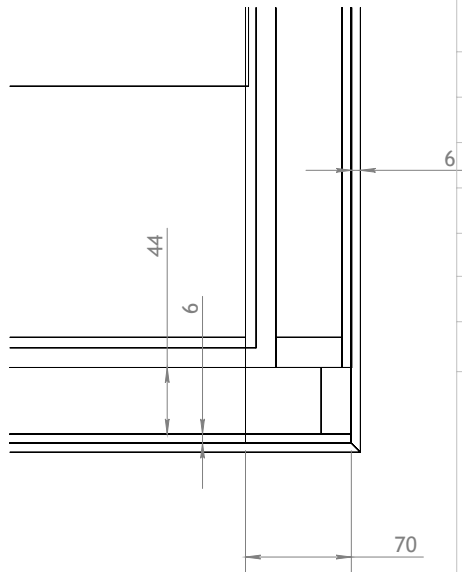
DETAIL D SCALE 1 : 5
