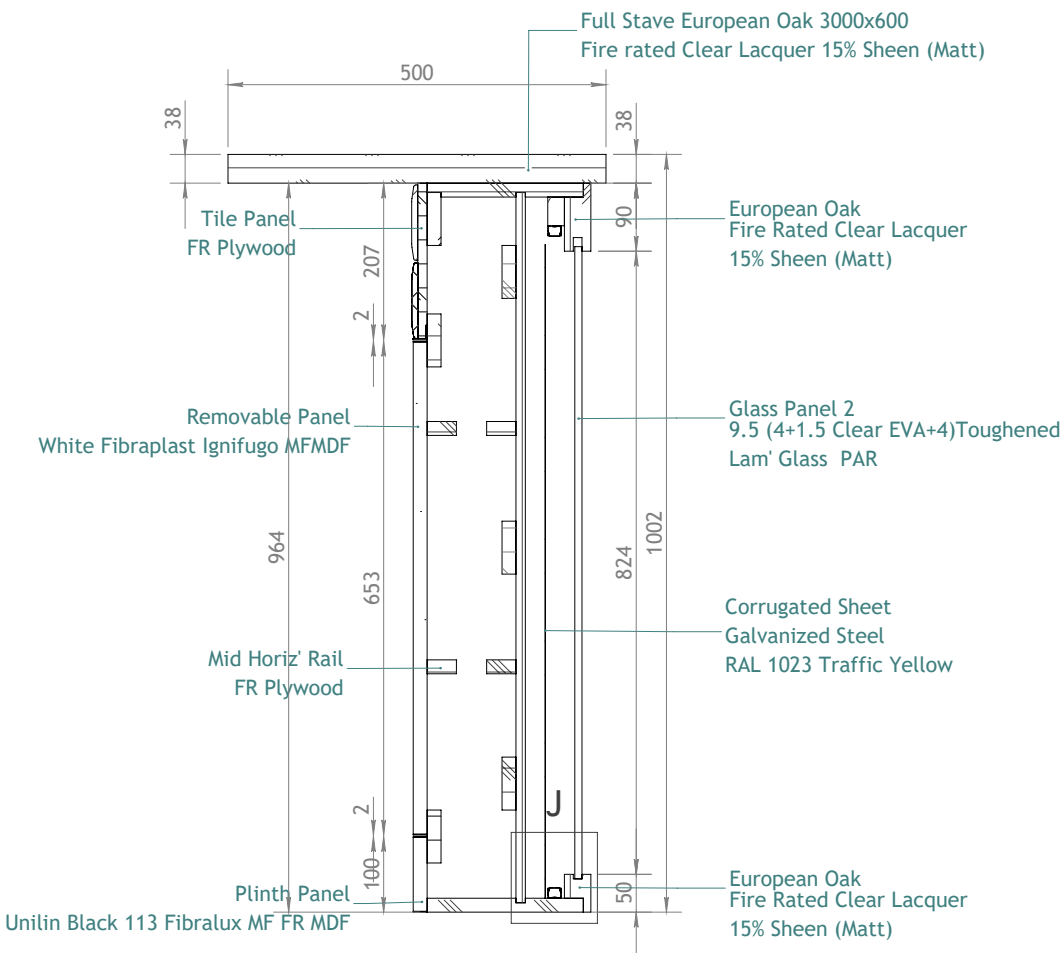
SECTION B-B
