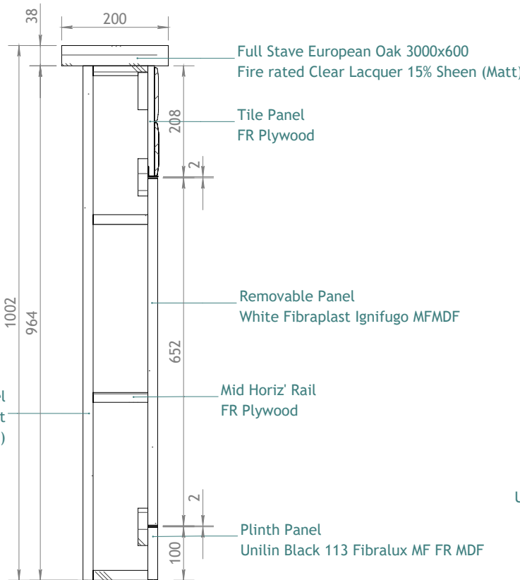
SECTION E-E
