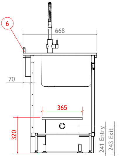
SECTION U-U
