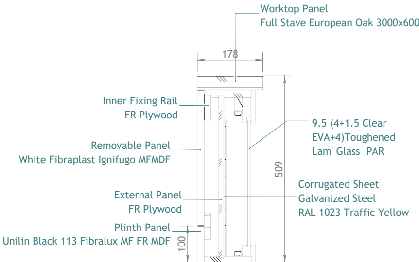
SECTION F-F
