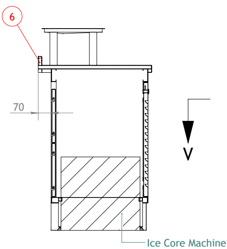
SECTION U-U
